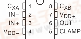
D014, J, OR N PACKAGE (TOP VIEW)
